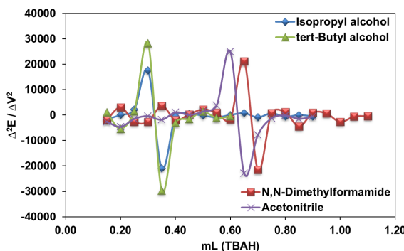
Figure 5. \Delta^2 E/\Delta V^2 -mL (TBAH) potentiometric titration curves of 0.001 M solutions of compound 5 titrated with 0.05 M TBAH in isopropyl alcohol, N,N -dimethyl formamide, tert -butyl alcohol and acetonitrile at 25 °C.
