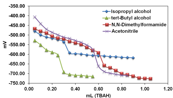
Figure 3. mV-mL (TBAH) potentiometric titration curves of 0.001 M solutions of compound 5 titrated with 0.05 M TBAH in isopropyl alcohol, N,N -dimethyl formamide, tert -butyl alcohol and acetonitrile at 25 °C.
